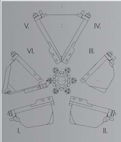
■ Arrangement of 6 independent cross slides
