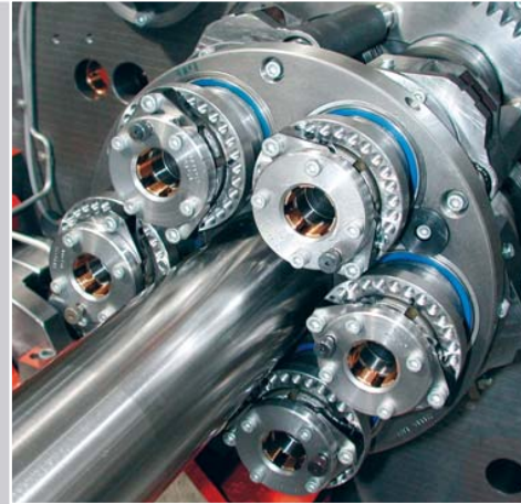
■ Back side of spindle drum with work spindles
