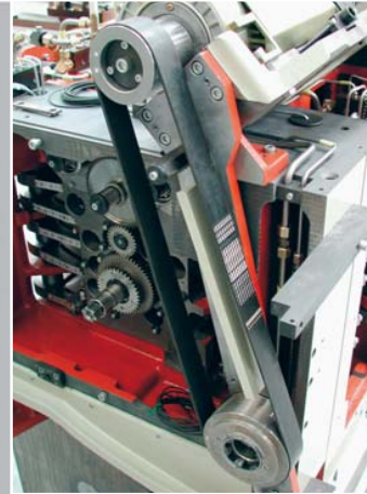
■ Tipping drive of working spindles enables an easy access to the interchangeable gear wheels of attachments and to the rocker arms of longitudinal and compound slides
