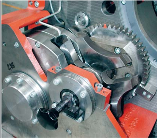
■ Geneva mechanism of spindle drum indexing. By the cam alterable length of arm ensures the high dynamics of indexing.
